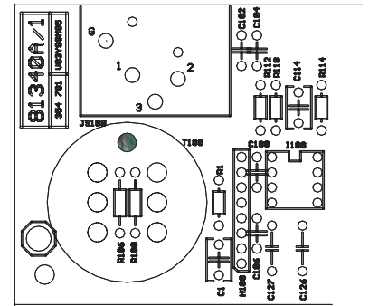
figure: printed board assembly area channel A – transformer retrofitting
