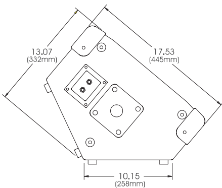
Figure 4—Dimension Line Drawing
