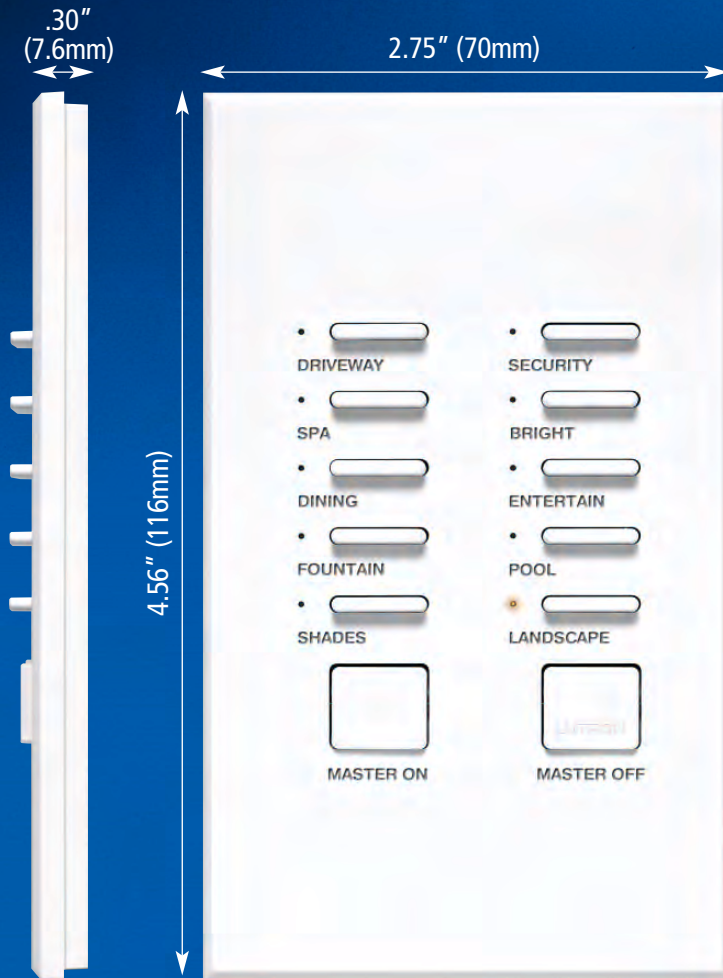
Shown actual size: Slim button style wallstation in white (WH).
